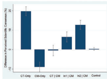
Note: CT = Consensus Treatment, CM = Coerce-Message, In1 = General Inoculation, In2 = Detailed Inoculation. Error bars represent 95% confidence intervals.
